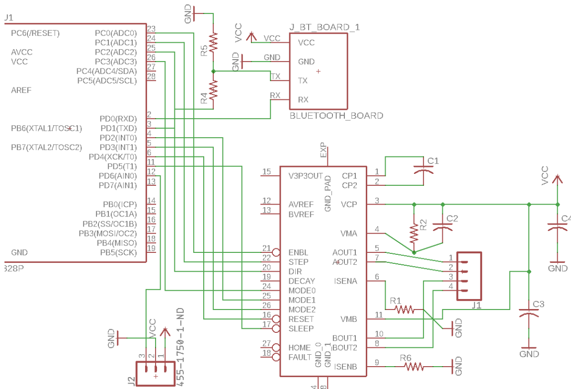
Figure 7-2: Preliminary Robofan Schematic
