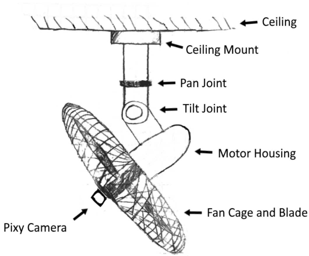
Figure 7-1; Robofan Prototype Sketch with Labeling
