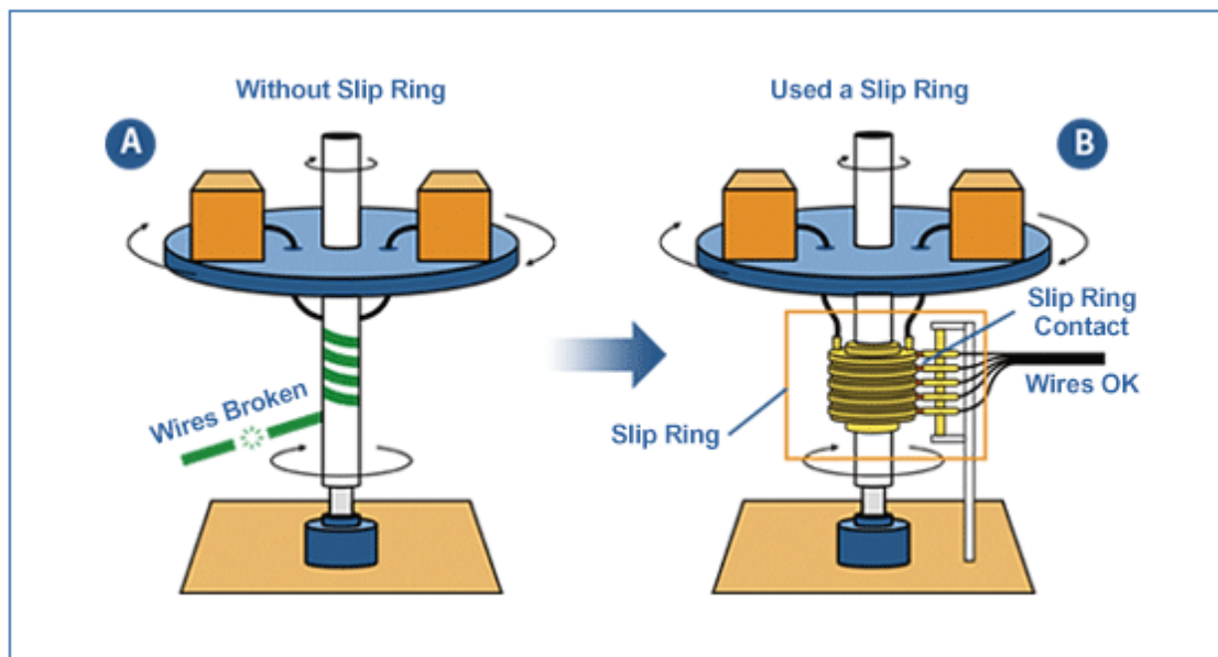
Figure 6-6: Diagram of Slip Ring (Pending Permission from Moflon)
