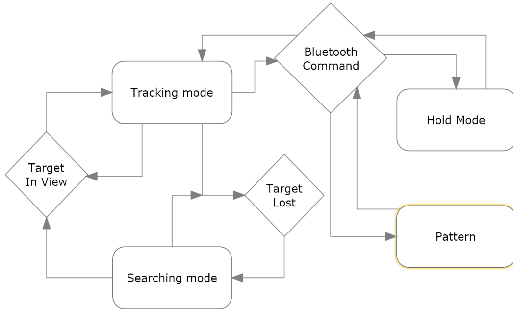
Figure 6-11: Mode Flowchart
