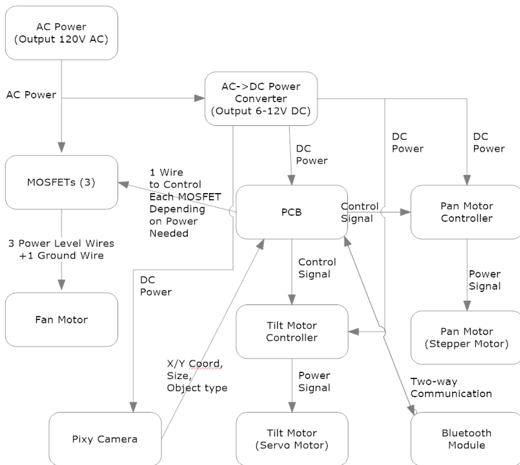
Figure 6-2: Hardware Wiring Diagram
