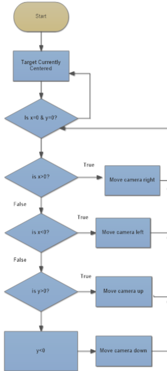
Figure 6-13: Servo Motor Flowchart
